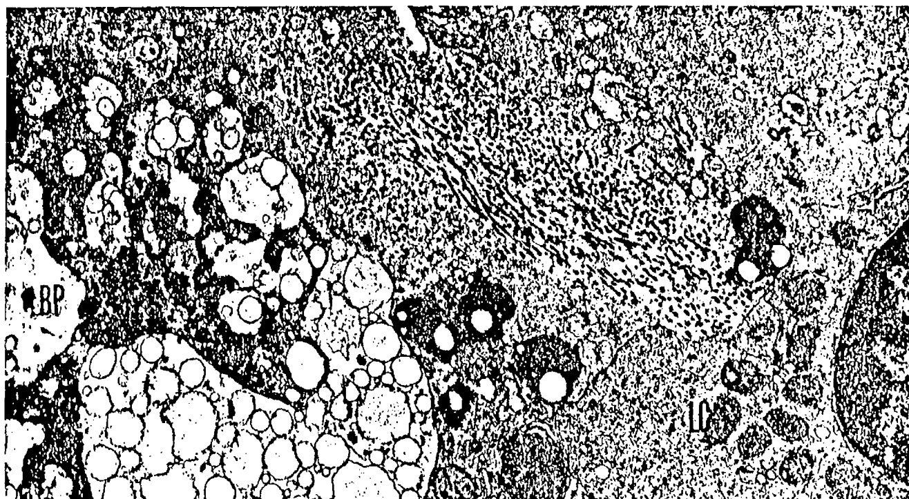
Fig 5. - Border of area of adenofibrosis in liver. Note round clusters of dark granules intermixed with web-like clusters of vacuoles. These formations illustrate appearance of brown pigment (BP). C represents collagen; LC, liver cell (lead citrate-uranyl acetate, original magnification \times 20,235 ).
