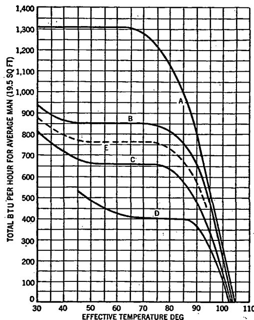
FIG. 5. RELATION BETWEEN TOTAL HEAT LOSS FROM THE HUMAN BODY AND EFFECTIVE TEMPERATURE FOR STILL AIR 14
