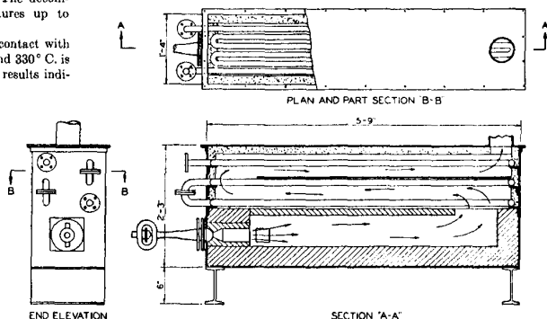
Figure 1. Heater
