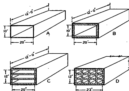
FIG. 6. ACOUSTIC TREATMENT OF DUCTS
