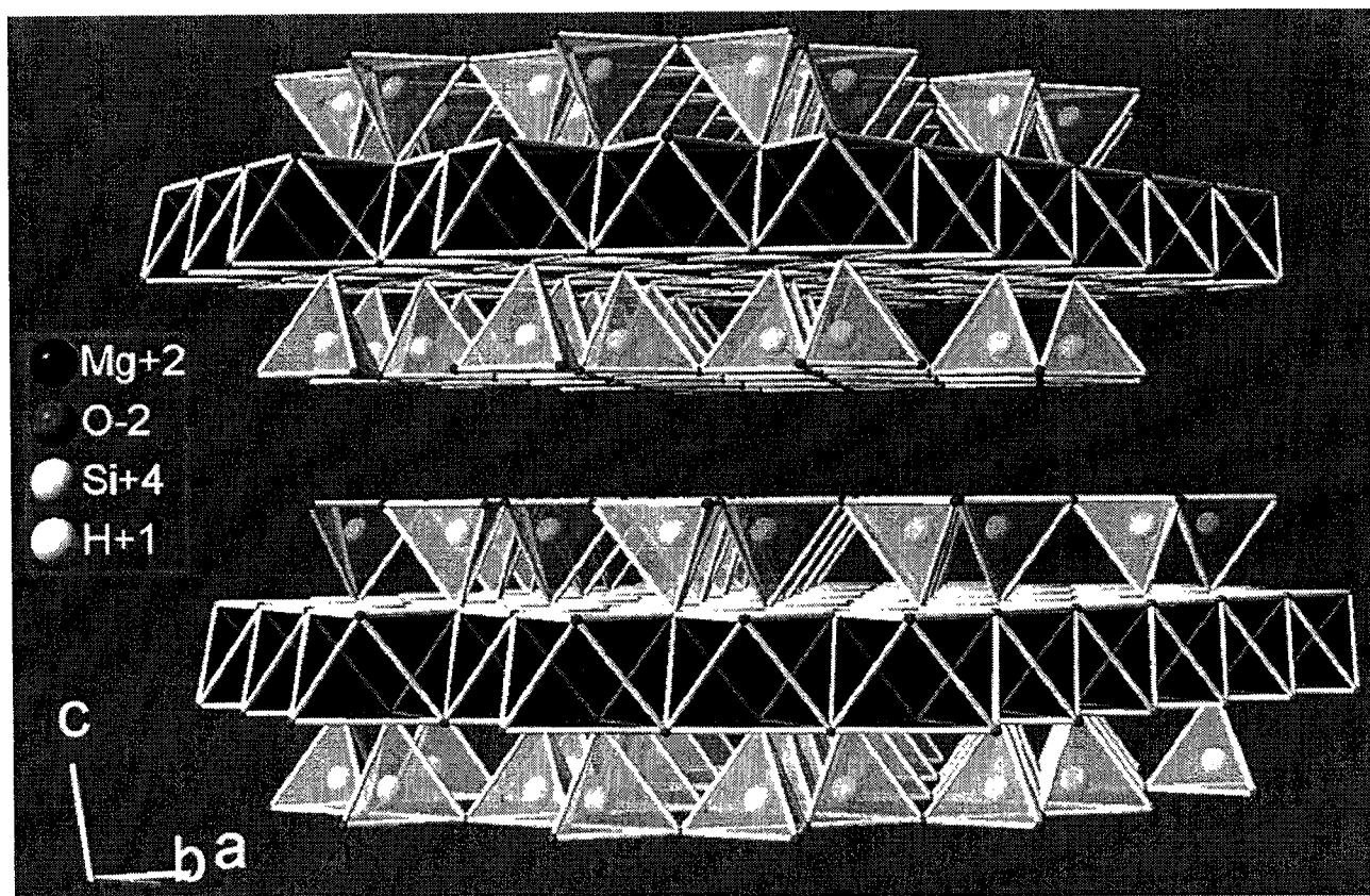
Figure 1.1 Schematic structure of talc
