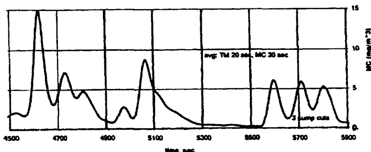
Figure 4. Dust concentrations measured by the MMRDM on 21 August 1995.
