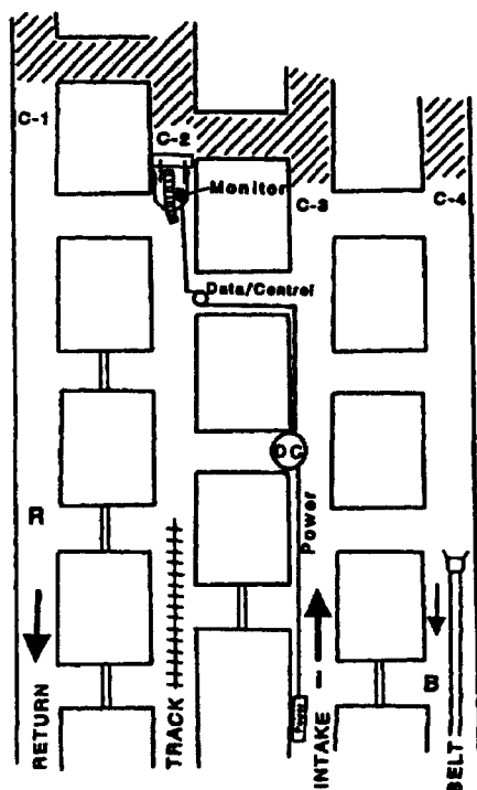
Figure 3. Location of MMRDM sensor (Monitor) and auxiliary electronics (DC) during phase one evaluation.
