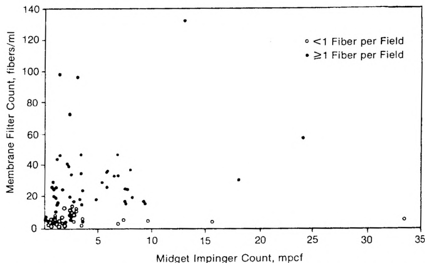
A plot of membrane filter and midget impinger counts; mpcf represents millions of particles per cubic foot.
