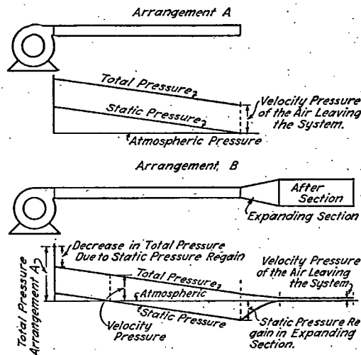
FIG. 6. APPLICATION OF STATIC PRESSURE REGAIN TO A SIMPLE FAN AND DISCHARGE DUCT
