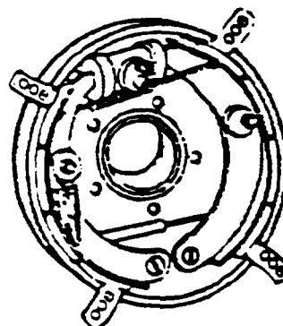
Lockheed Hydraulic
