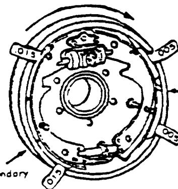
Bendix Dual-Servo
