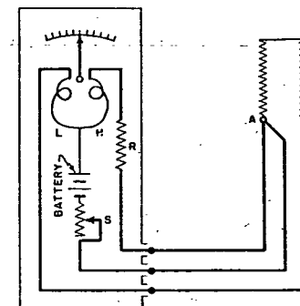
FIG. 2. TYPICAL RESISTANCE THERMOMETER CIRCUIT AND CONNECTIONS
