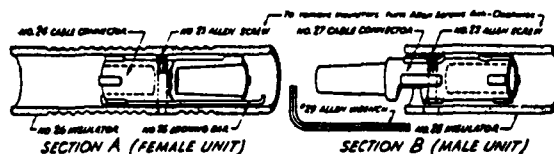
To assemble, insert apart as shown by arrows ASSEMBLED UNITS
