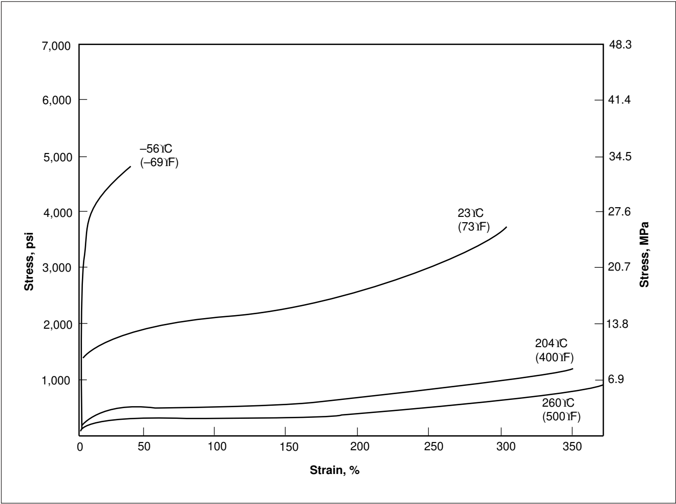
Figure 2b. Stress vs. Strain in Tension
