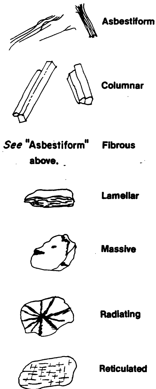
FIGURE 21. - Various shapes of single crystals, and patterns or arrangements of crystal aggregates.
