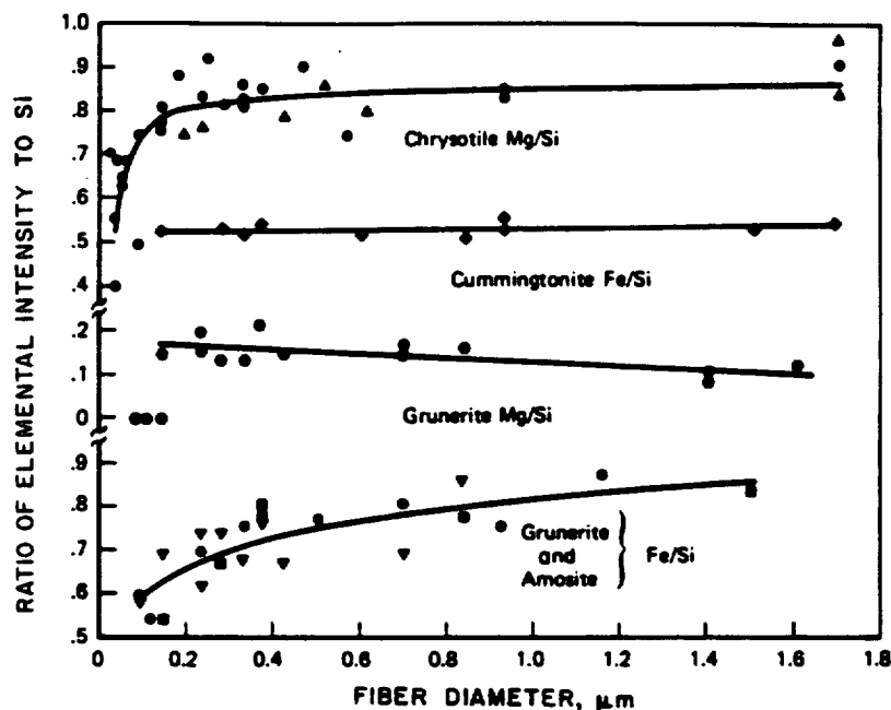
FIGURE 34. - Intensity ratio of \text{FeK}\alpha , \text{MgK}\alpha , or \text{CaK}\alpha relative to \text{SiK}\alpha as a function of fiber diameter. (Reprinted with permission of D. R. Beaman and D. M. File from Analytical Chemistry (2). Copyright by the American Chemical Society.)
