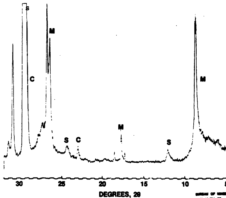
FIGURE 49. - X-ray diffractometer scan of sample from school ceiling, showing the presence of calcite (C), mica (M), and serpentine (S).
