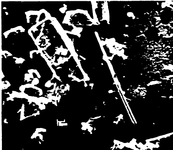
FIGURE 53. - Platy talc, tremolite cleavage fragments, and a fibrous tremolite particle (A) (X 400).
