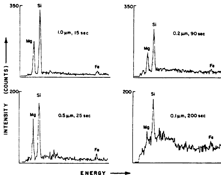
FIGURE 36. - Energy-dispersive X-ray spectra of chrysotile as a function of fiber diameter, Be substrate (21).
