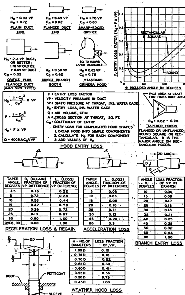
FIG. 2. EXHAUST SYSTEM DESIGN DATA 13
