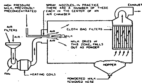
FIG. 15. SPRAY DRYER OF THE PRESSURE-SPRAY ROTARY TYPE 9
