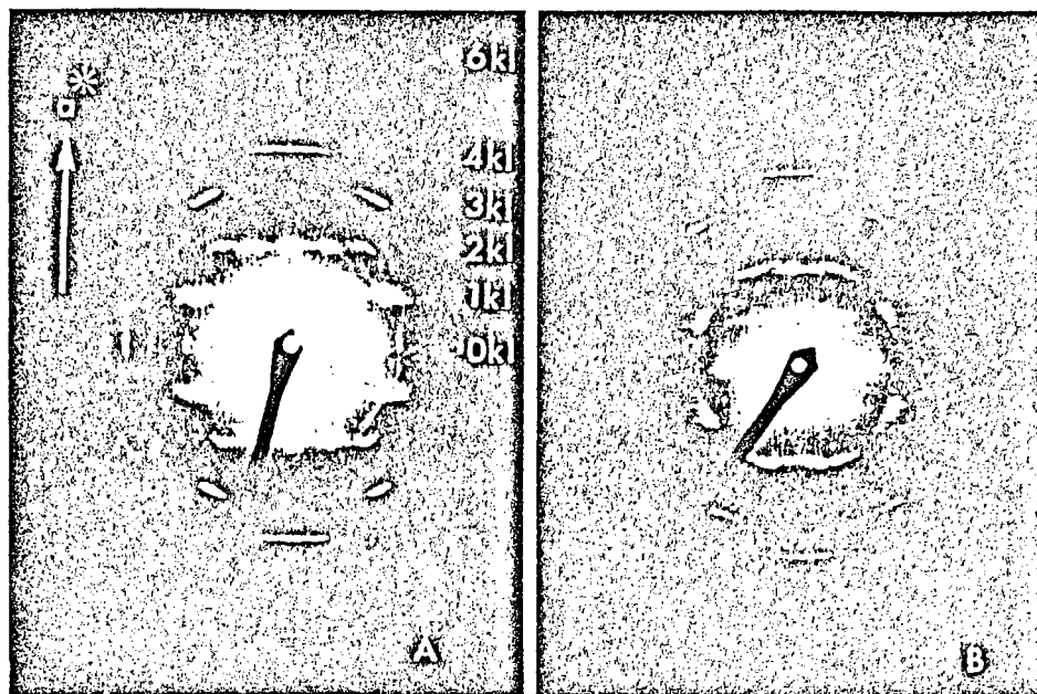
FIG. 2. Selected area electron diffraction patterns obtained on fibers of chrysotile obtained during air sampling at brake repair shops. In A, the reciprocal a axis is marked a* as are the layer lines in the (OKI) series. Indexing of upper right quadrant yielded 16 reflections corresponding to single crystal X-ray diffraction analysis of Whittaker and Zussman, 1956. Pattern in (B) displays "smearing" of reflections in a "clockwise" manner suggesting interplanar rotation.
