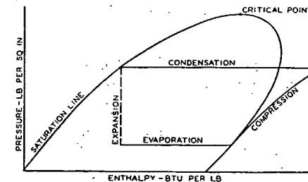
FIG. 4. PRESSURE-ENTHALPY DIAGRAM FOR SIMPLE SATURATION CYCLE
