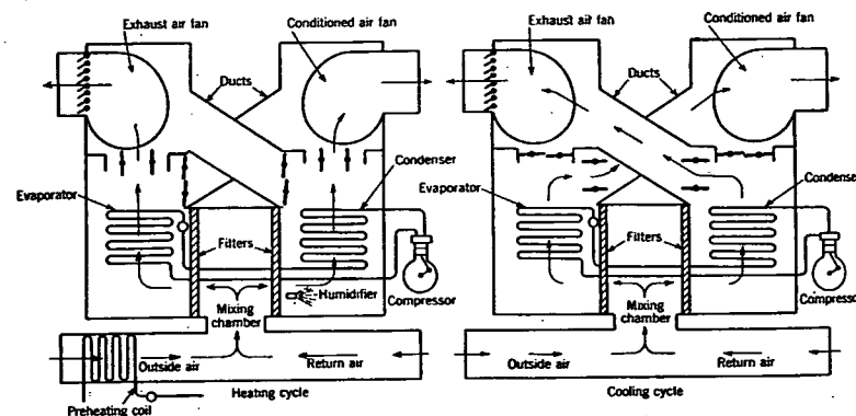
FIG. 10. SCHEMATIC OPERATION OF REVERSED CYCLE CONDITIONING SYSTEM
