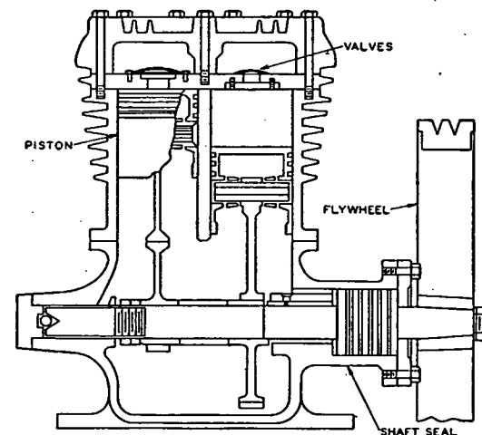
FIG. 11. DIAGRAMMATIC VIEW OF A RECIPROCATING COMPRESSOR
