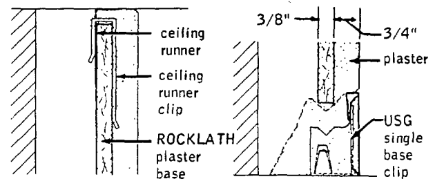
ceiling attachment
