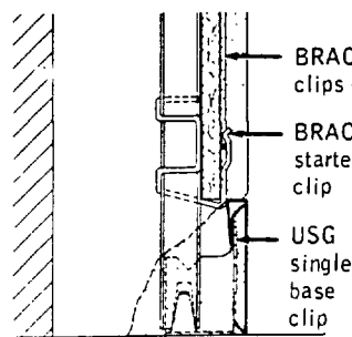
metal base
