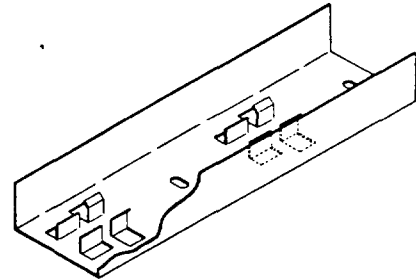
USG floor runner & screed
