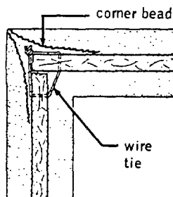
corner
