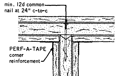
partition intersection
