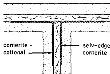
partition intersection
