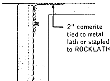
ceiling attachment
