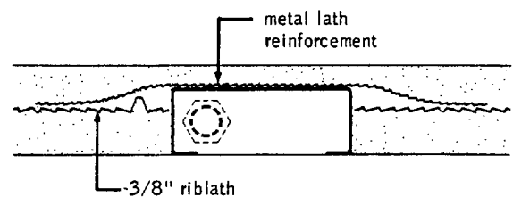
outlet box
