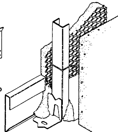
USG floor runner & screed
