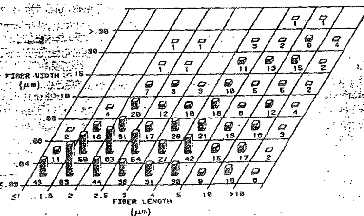
FIG. 6. Fiber size distribution for fibers extracted from five rats of the 24-month (terminal) sacrifice.
