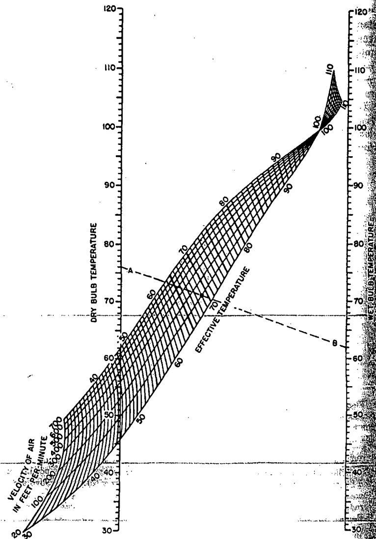
Figure 3. Normal scale of effective temperature applicable to inhabitants of the United States wearing customary clothing, at rest or doing light physical work, and in rooms heated by convection methods. (Reprinted by permission from Heating, Ventilating, Air Conditioning Guide , 1957, Chapter 6.)
