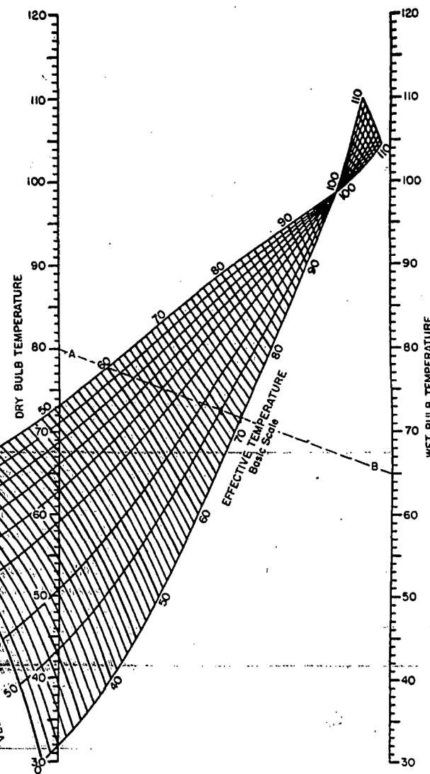
Figure 4. Basic scale of effective temperature applicable to men stripped to the waist, at rest or doing light physical work, and in rooms heated by convection methods. (Reprinted by permission from Transactions ASHVE , Vol. 38, 1932, Report No. 933.)
