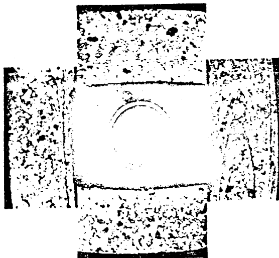
Fig. 8. Grain Structure of F-3 Sheath Sample No. 9 After Laboratory Heat Treatment
