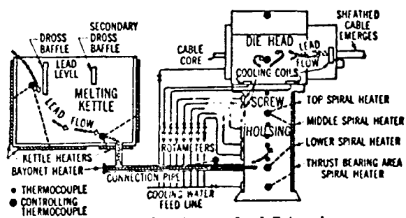
Fig. 1. Continuous Lead Extrusion Machine
