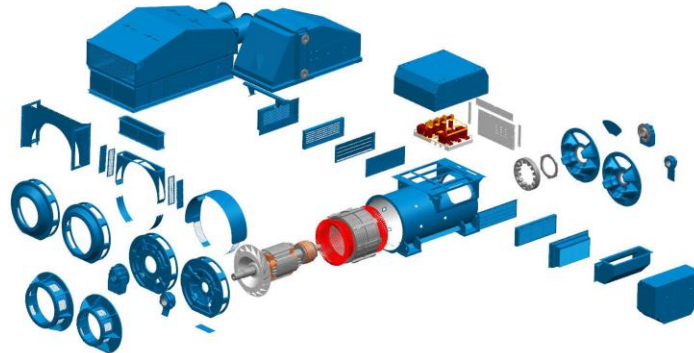
Figure 9 - exploded view of pre-engineered configurations for customisation of a compact high-voltage generator (2 p. 28)
