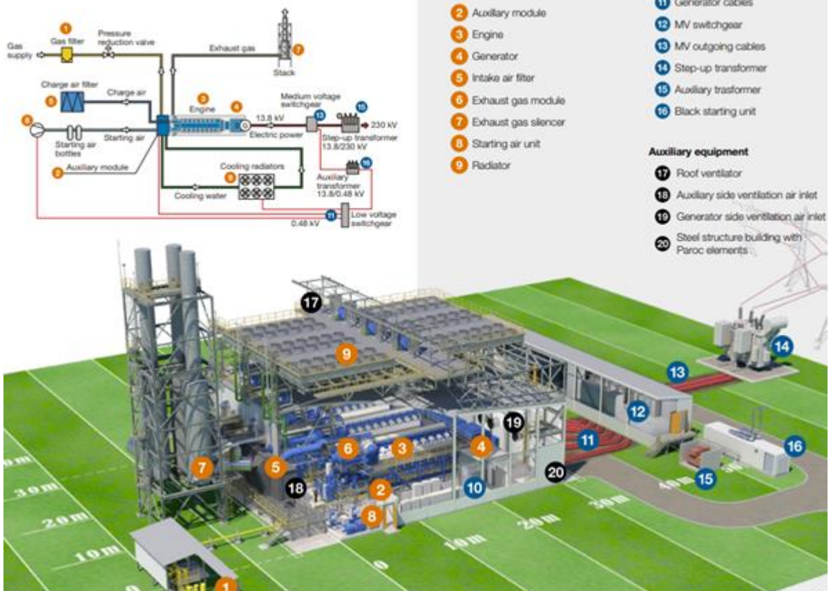
Figure 2 - schema of Combined Heat & Power system (18 p. 56)
