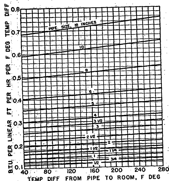
FIG. 3. HEAT LOSS THROUGH 2 IN. THICK 85 PERCENT MAGNESIA TYPE COVERING
