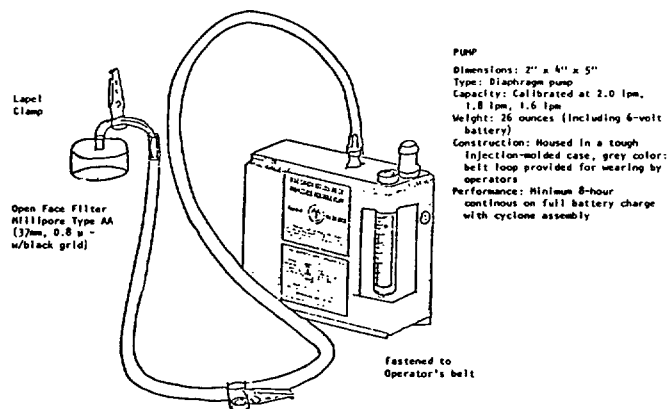
FIGURE 2. ASBESTOS SAMPLER
