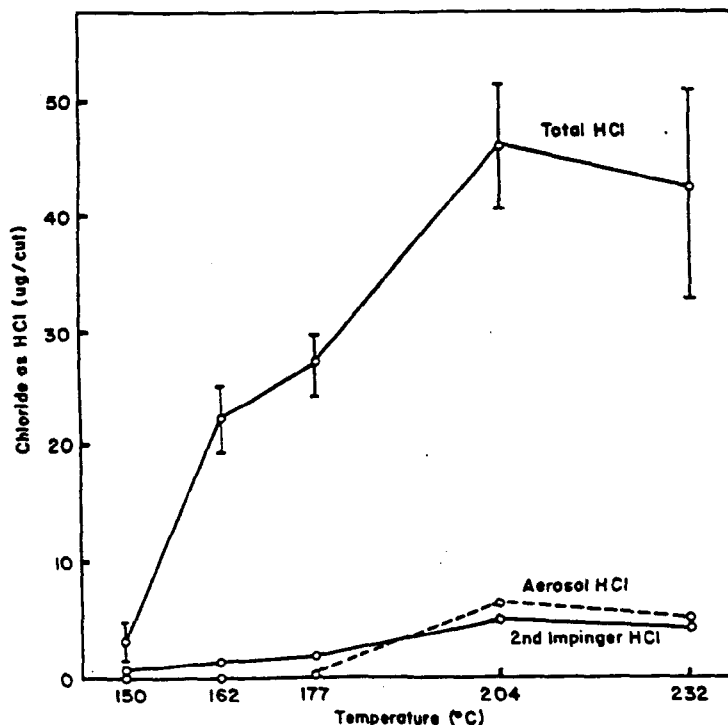
Figure 6 — Emissions of total chloride (as HCl), aerosol chloride and chloride collected in the second impinger as a function of temperature.
