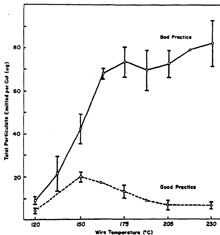
Figure 3 — Total particulate emissions as a function of wire temperature and cutting technique.
