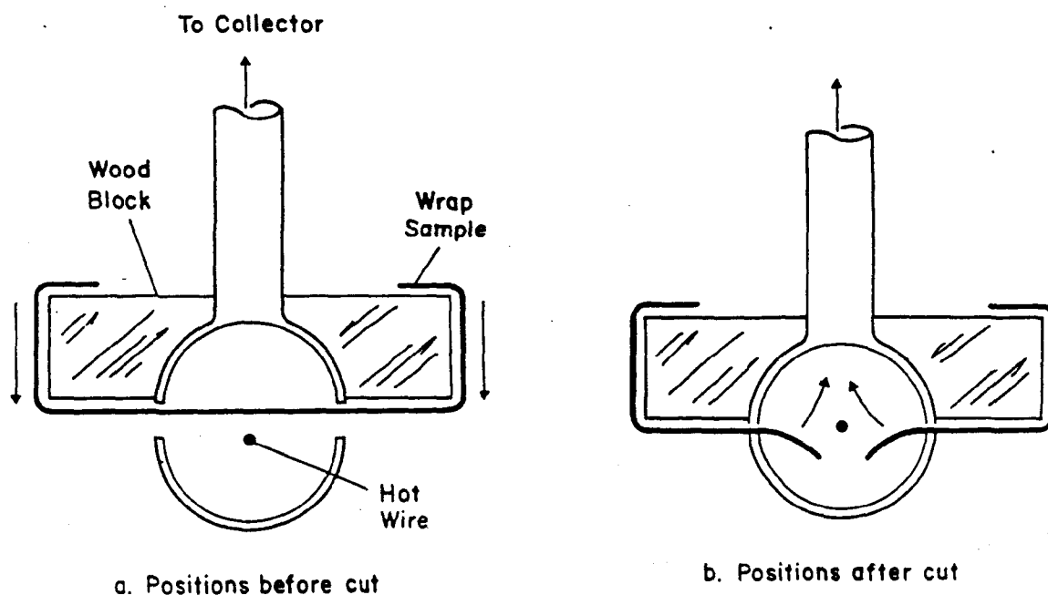
Figure 2 — Diagram of the glass hood for collecting the emissions from wire cutting.
