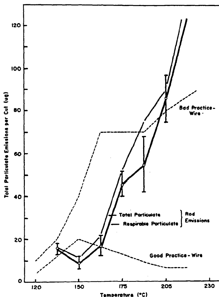
Figure 4 — Total and respirable particulate emissions as a function of temperature.
