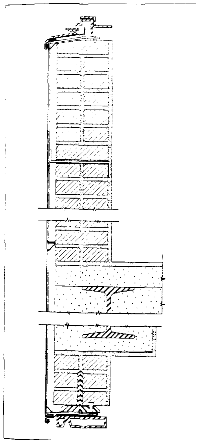
Section of the lead spandrel.
