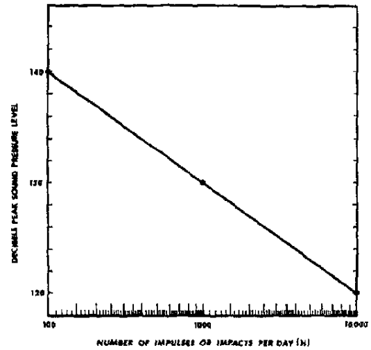
Figure 7 — Threshold Limit Values for Impulse/Impact Noise.
