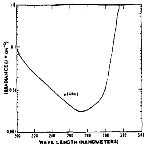
Figure 8 — Threshold Limit Values for Ultraviolet Radiation
