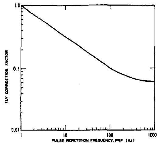
Figure 6 — Multiplicative correction factor for repetitively pulsed lasers having pulse durations less than 10 -4 second. TLV for a single pulse of the pulse train is multiplied by the above correction factor. Correction factor for PRF greater than 1000 Hz is 0.06.
