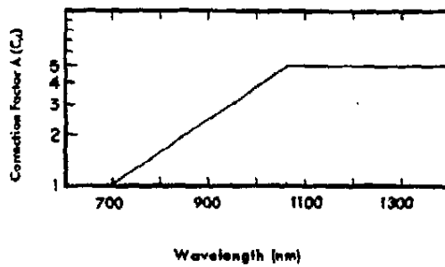
Figure 2 — TLV correction factor for \lambda = 700 - 1400 \text{ nm}^*
