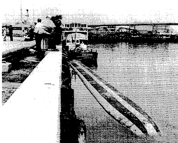
Partially unloaded and collapsed Dracone at Esso terminal on Whale Creek, Brooklyn. For return trip container was inflated with CO 2 .
