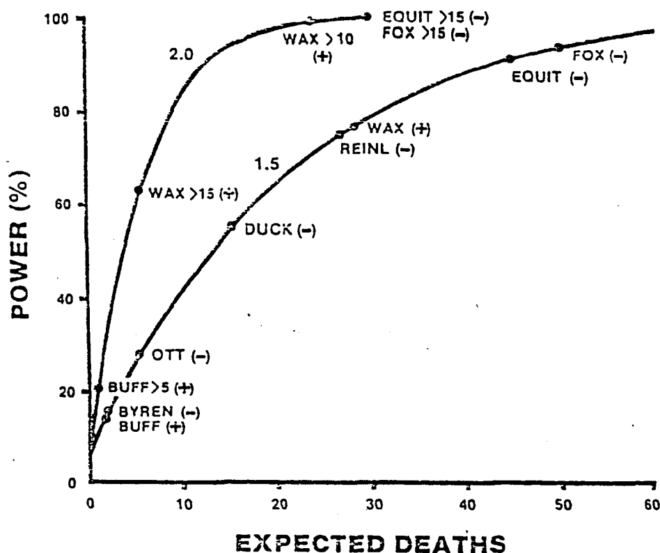
FIGURE 4. Approximate powers of vinyl chloride studies reporting results for lung cancer: 2.0 = assumed relative risk after a minimum latency, 1.5 = assumed relative risk overall. BUFF = Buffer et al. (9); BYREN = Byren et al. (11); OTT = Ott et al. (10); DUCK = Duck et al. (12); REINL = Reini et al. (8); WAX = Waxweiler et al. (4, 5); EQUIT = Equitable Environmental Health (6, 7); FOX = Fox and Collier (1, 2).
