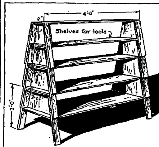
HANDY ladder from sawhorses clamped together.
