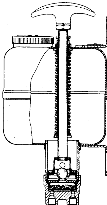
FIG. 3 SECTIONAL VIEW OF BIJUR LUBRICATOR
