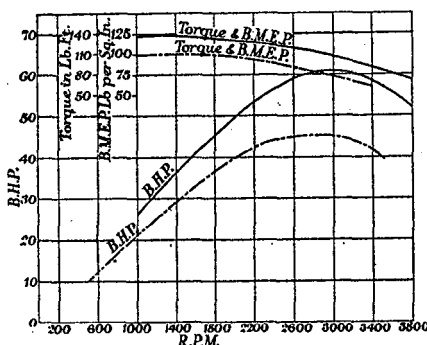
FIG. 2 POWER AND TORQUE CURVES OF A WOLF AIRLESS-INJECTION ENGINE FOR MOTOR VEHICLES
