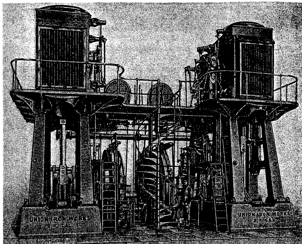
DOUBLE 26 IN. AND 46 X 72 IN. HOISTING ENGINE (Anaconda Mining Co., Butte, Montana.)
