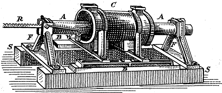
SKETCH OF WILKINSON'S BORING MACHINE USED FOR MACHINING CYLINDERS OF WATT'S ENGINE
