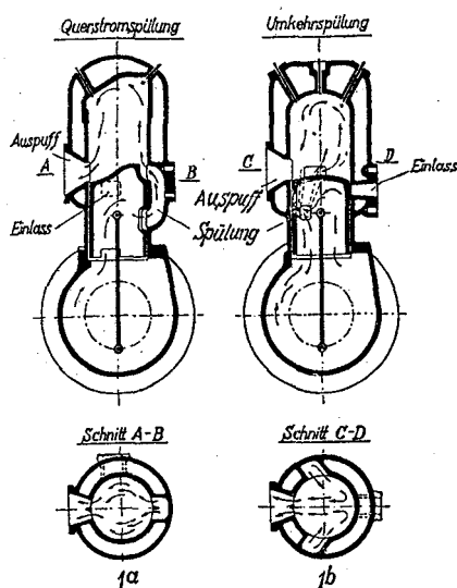
FIG. 1 DIAGRAMMATIC PRESENTATION OF THE CONVENTIONAL AND NEW METHODS OF SCAVENGING TWO-STROKE-CYCLE HIGH-SPEED CARBURETOR ENGINES
