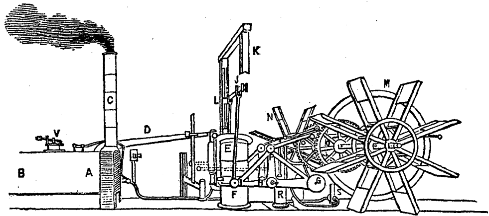
THE ENGINES OF THE "CLERMONT" (From Thurston's "History of the Steam Engine.")
