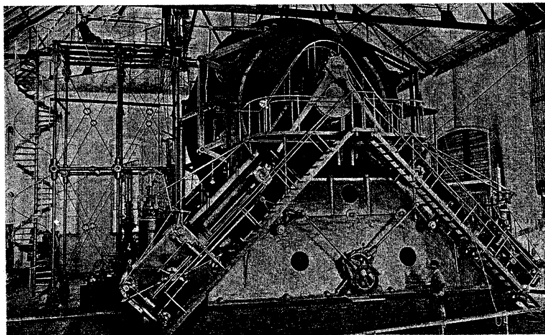
TAMARACK HOIST—MICHIGAN
