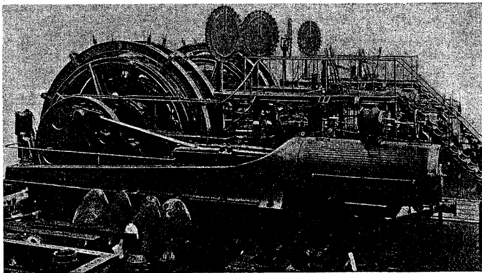
DOUBLE 30 X 72 IN. HOISTING ENGINE (Anaconda Mining Co., Butte, Mont.)
