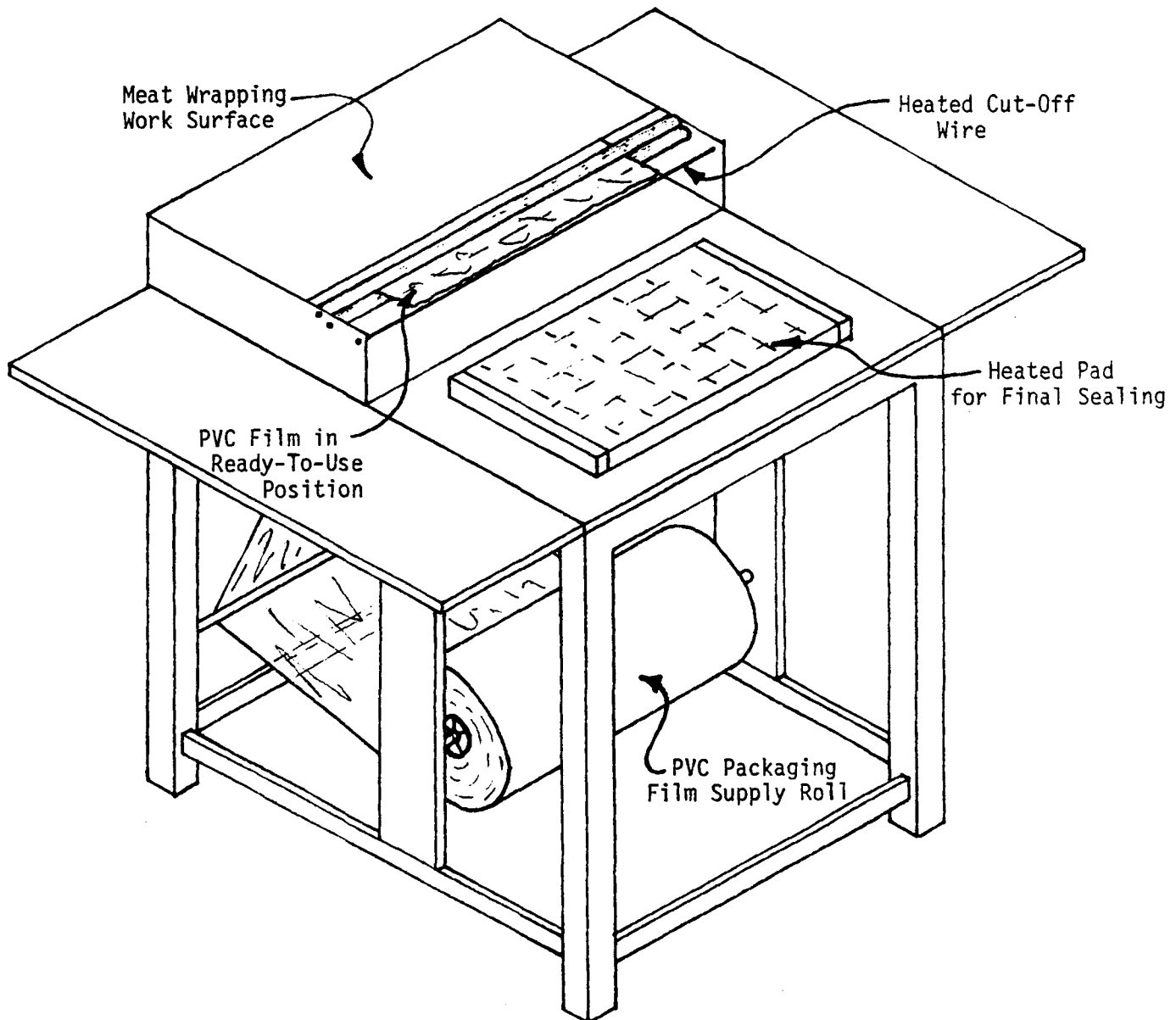
FIGURE 1: Typical Hand-Wrapping Machine
