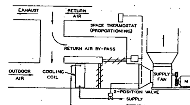
Fig. 20.... Control of Chilled Water Coil from Space Temperature Using Return Bypass Damper and Valve
