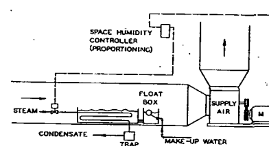
Fig. 21.... Control of Pan Humidifier
