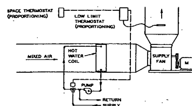
Fig. 18.... Control of Hot Water Coil from Space and Discharge Air Using Mixing Valve
