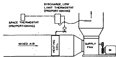
Fig. 16.... Control of Heating Coil from Space and Discharge Air Using Valve
