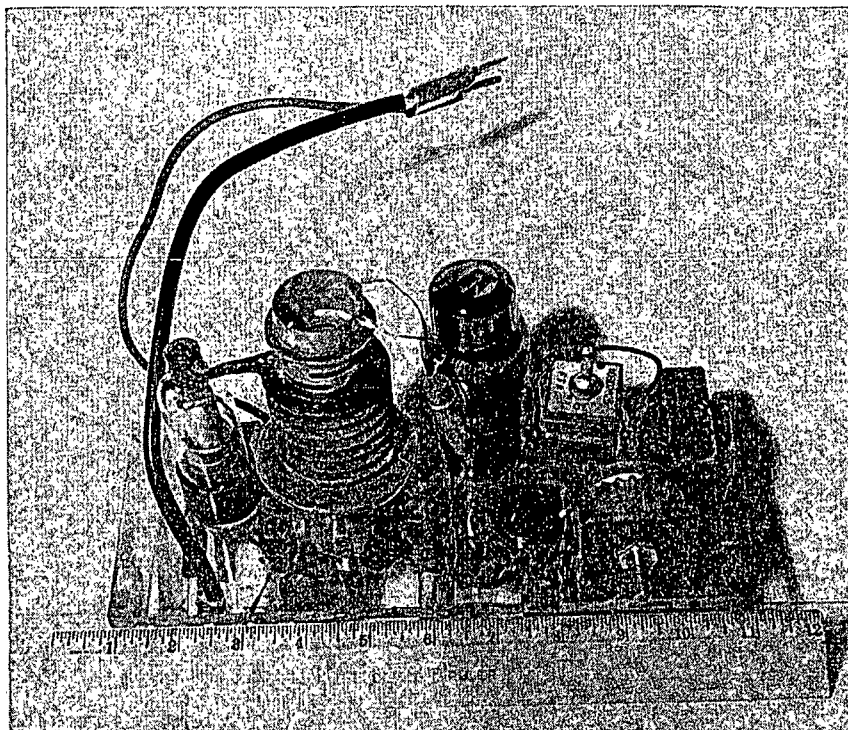
Fig. 1.—The PHS-50 high voltage power supply.
