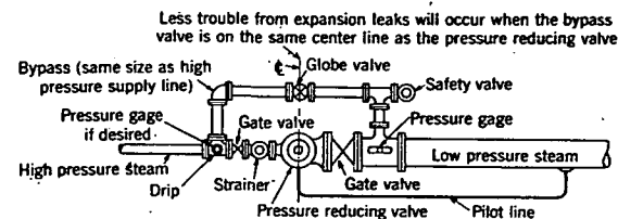
FIG. 2. TYPICAL PRESSURE REDUCING VALVE INSTALLATION
