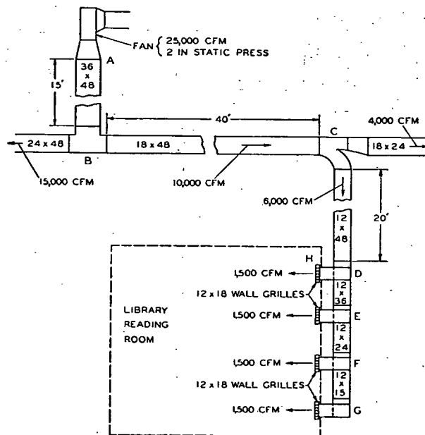
FIG. 19. ASSUMED VENTILATING SYSTEM FOR EXAMPLE 3
