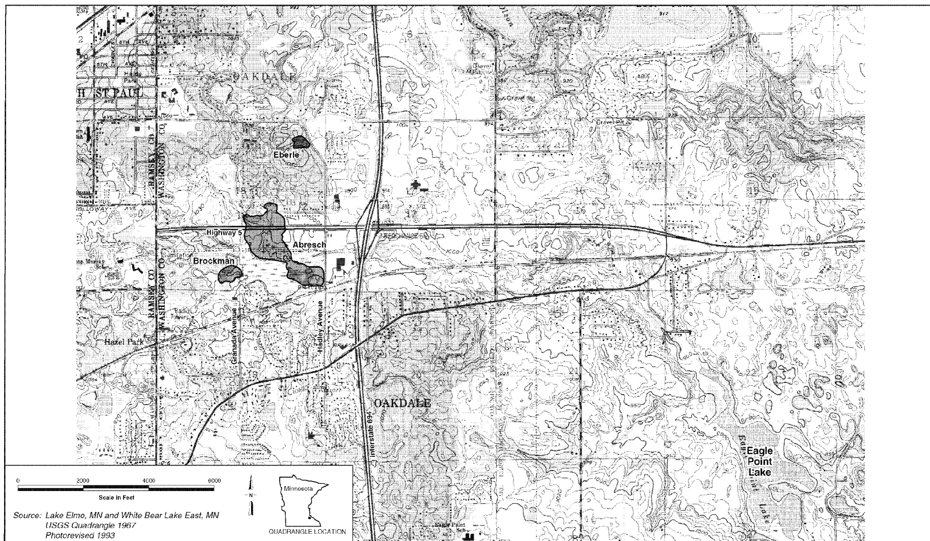
FIGURE 1 SITE LOCATION MAP OAKDALE SITE, MN
