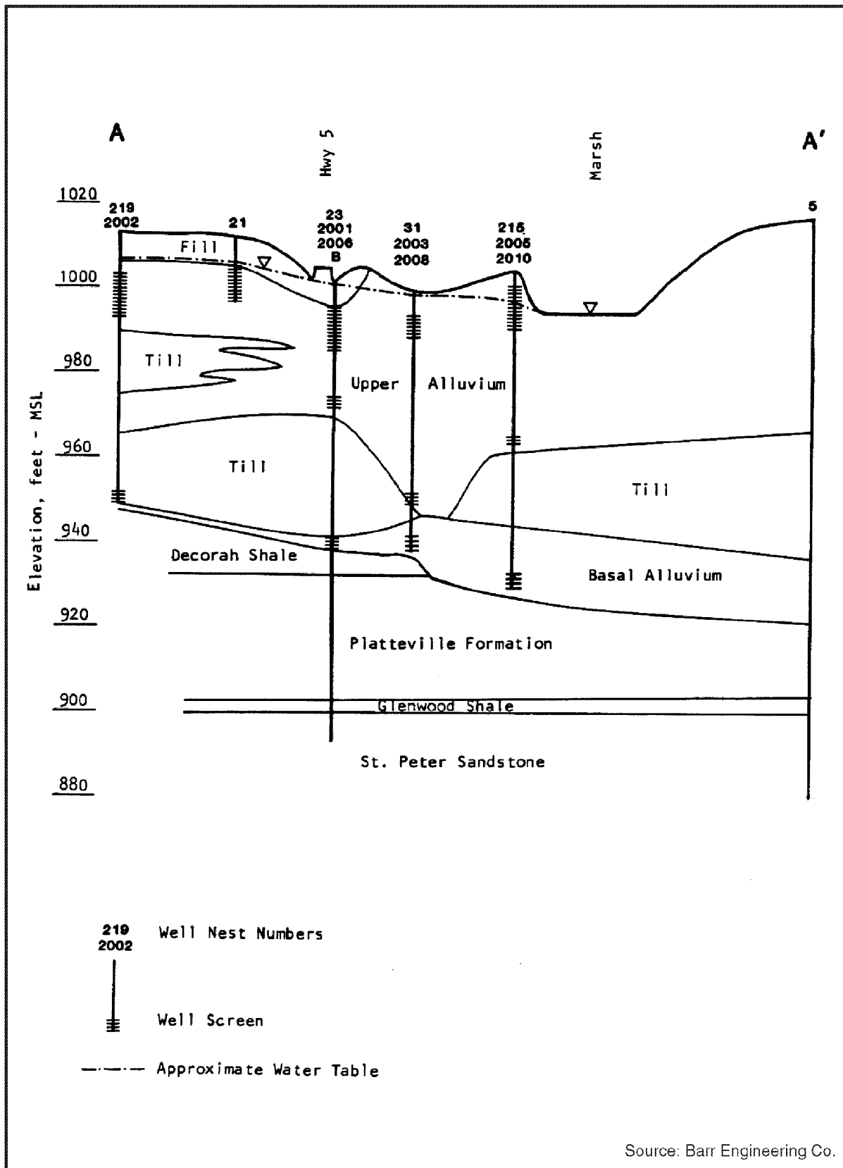
FIGURE 3 GEOLOGIC CROSS SECTION A-A' OAKDALE SITE, MN
