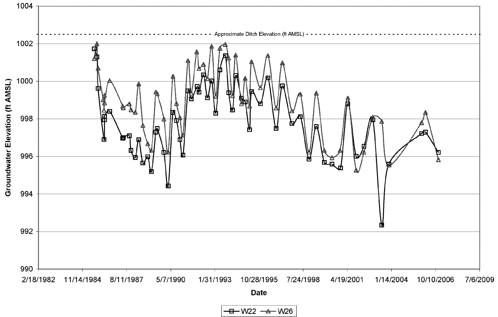
Figure 8 W22 and W26 Hydrograph and Approximate Drainage Ditch Elevation Oakdale, MN
