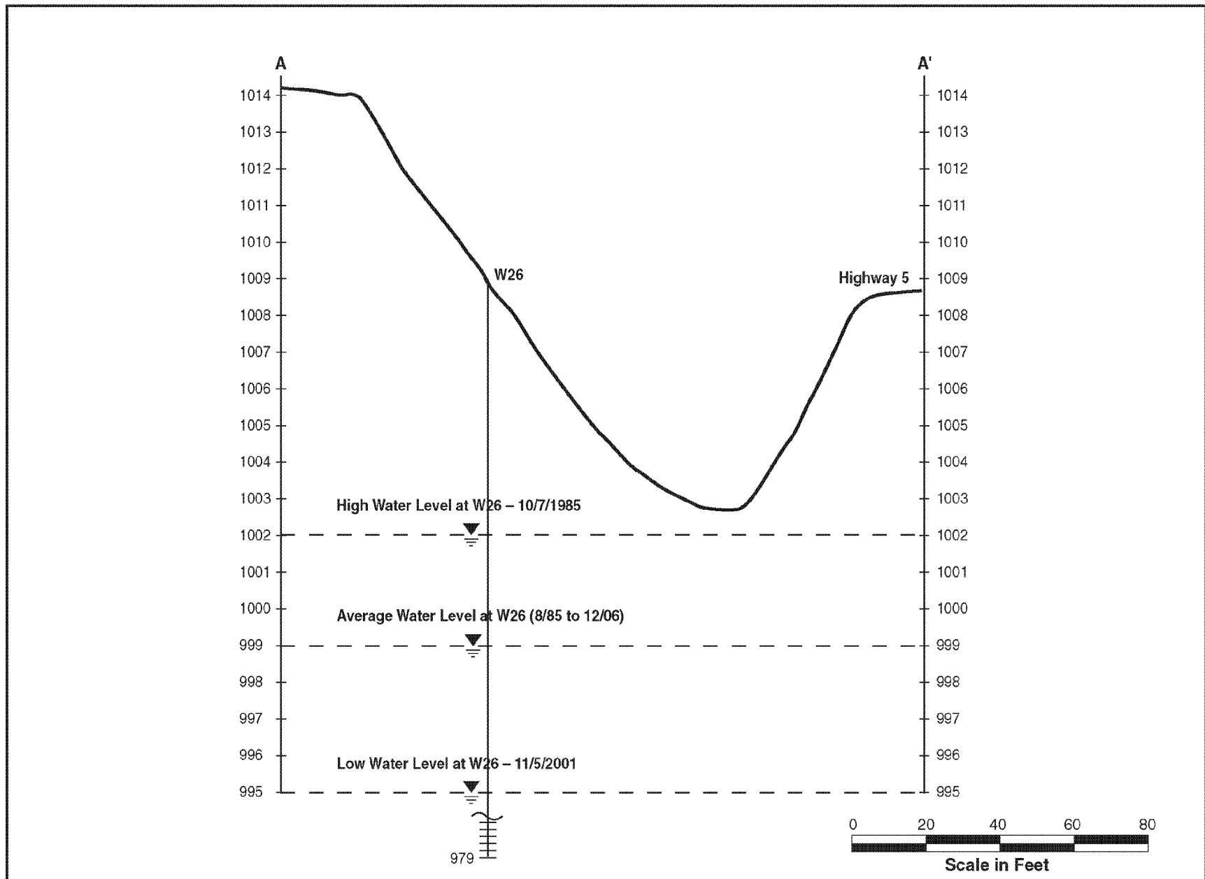
FIGURE 9 CROSS SECTION A-A' - WATER LEVEL ELEVATIONS AT MONITORING WELL W26 OAKDALE, MN
