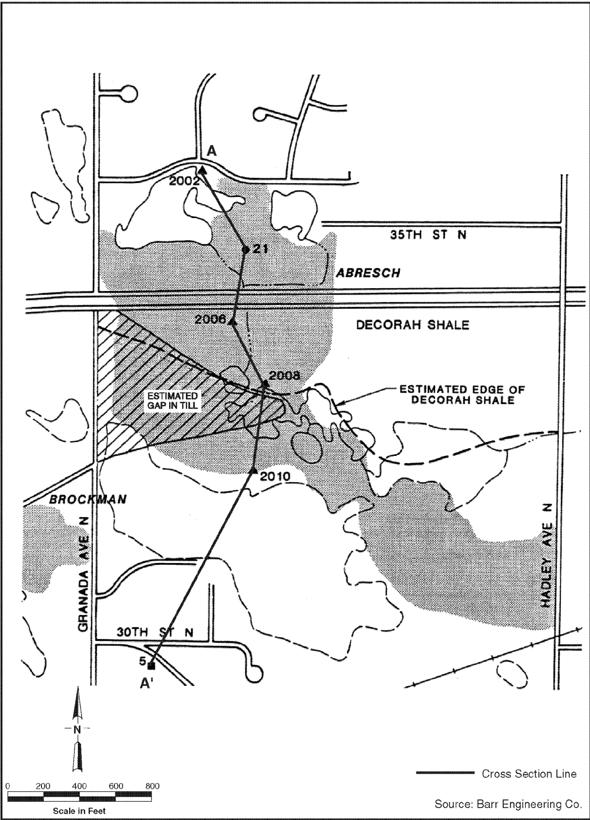
FIGURE 2 ESTIMATED GAP IN TILL AND EDGE OF DECORAH SHALE
