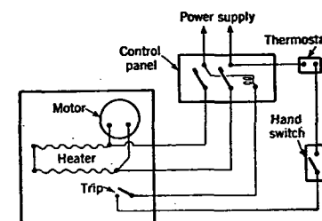
FIG. 1. WIRING DIAGRAM FOR UNIT HEATER
