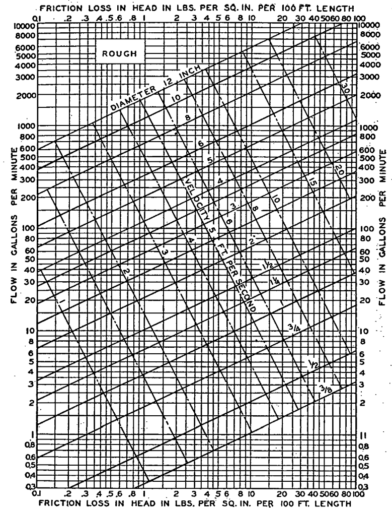
FIG. 4. FLOW CHART FOR ROUGH PIPE
