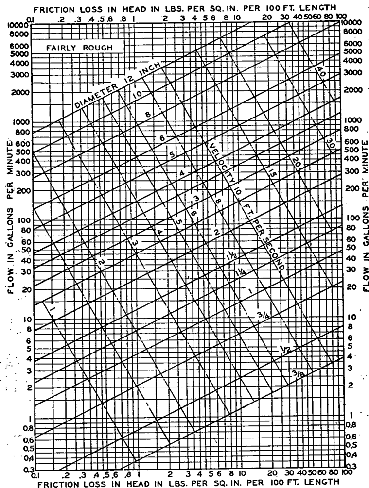
FIG. 3. FLOW CHART FOR FAIRLY ROUGH PIPE
