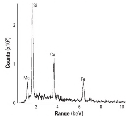
Figure 8. Seven examined uncoated fibers out of 20 showed the elemental composition of silicon, magnesium, calcium, and iron in a proportion indicative of actinolite.
