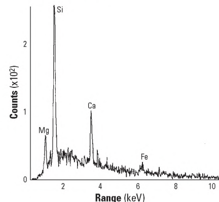
Figure 7. Energy dispersive spectra of case MM2 shows a large peak for silicon and two intermediate peaks for calcium and magnesium. This elemental composition is consistent with tremolite.
