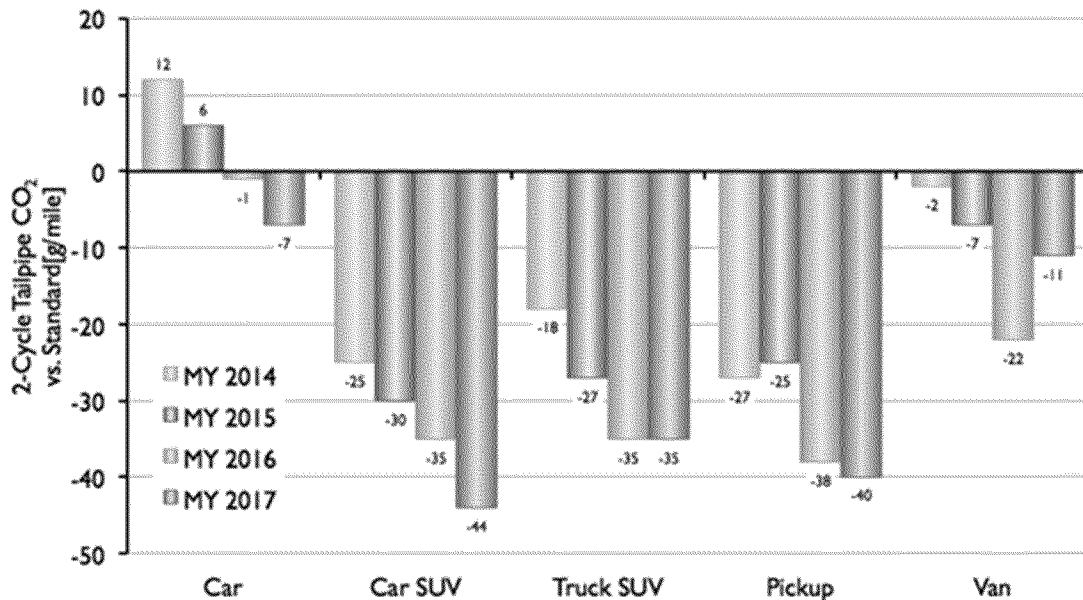
Figure 6.5: CO 2 performance-to-standard. 208
