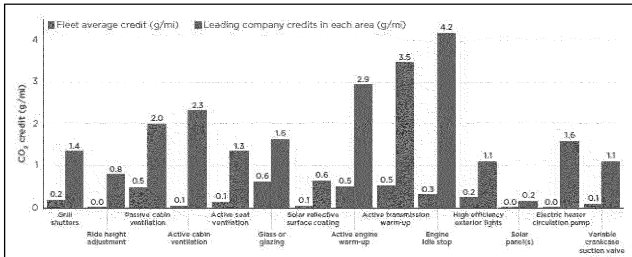
Figure 5.5: Data produced by ICCT representing the fleet-wide average and leading company credits for 14 technology areas used to justify the high scenario. 187 Of the 14 values for leading company credits, 12 are incorrectly cited.
