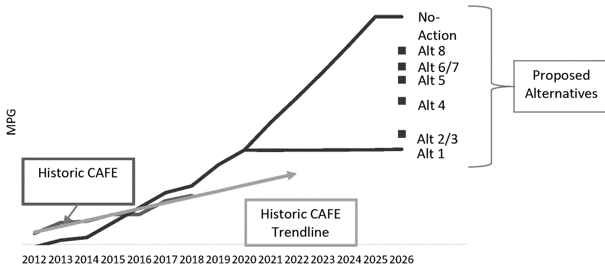
Figure 1.2: CAFE compliance performance improvements necessary to meet projected target values in MY 2026 (MY 2025 for the no-action alternative) starting from MY 2020. 15
