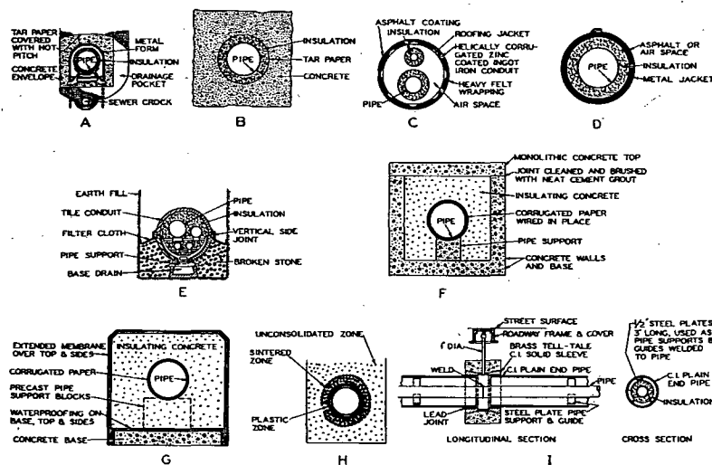
Fig. 1.... A Few Typical Conduits for District Heating Use
