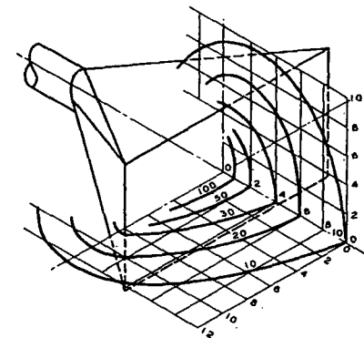
Fig. 1.... Velocity Contours for Rectangular Opening with a Side Ratio of One-Half. Contours are Expressed as Percentages of the Velocity at the Opening
