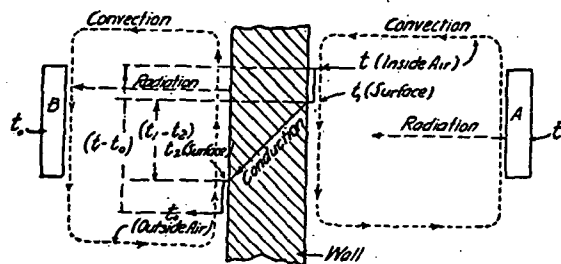
FIG. 1. TEMPERATURE CURVE OR GRADIENT FROM AIR INSIDE TO AND THROUGH WALL TO AIR OUTSIDE, WALL MATERIAL ASSUMED AIR-TIGHT
