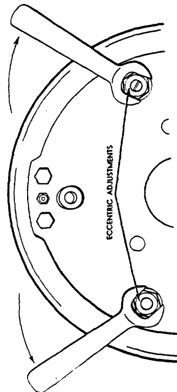
Figure 7B Method of adjusting eccentric cams on Lockheed Self-adjusting Brakes
