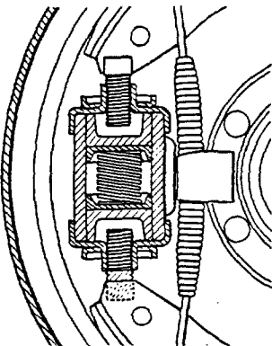
Figure 19 Sectional View of Hydraulic Wheel Cylinder on Huck Hydraulically Operated Brakes
