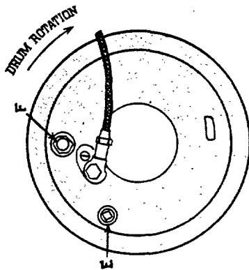
Figure 8 View from Backing Plate Side of Bendix Hydraulically Operated Brake
