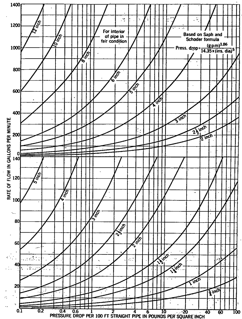
FIG. 3. CHART GIVING PRESSURE DROP FOR VARIOUS RATES OF FLOW OF WATER
