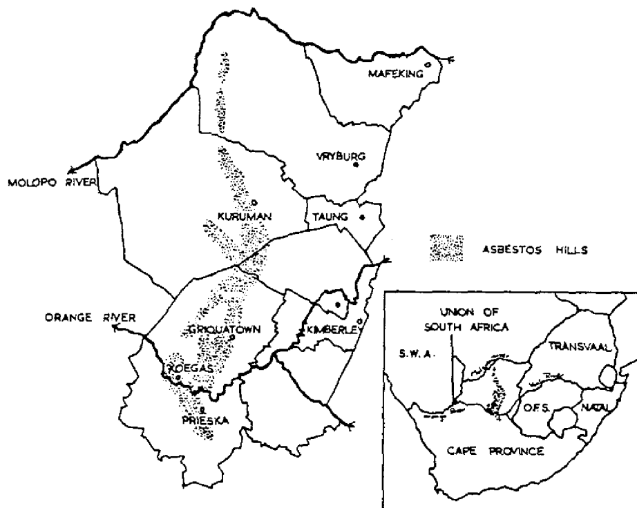
FIG. 1.—Map of Griqualand West asbestos fields.
