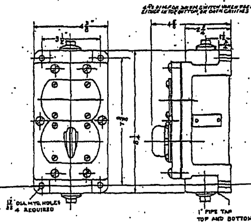
Two unit heavy duty master station with rotary drum switch element used in at least one unit. (Rotary drum switch element determines the maximum depth).
