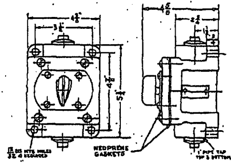
Single Unit Spraytight Rotary Drum Type Master Station
