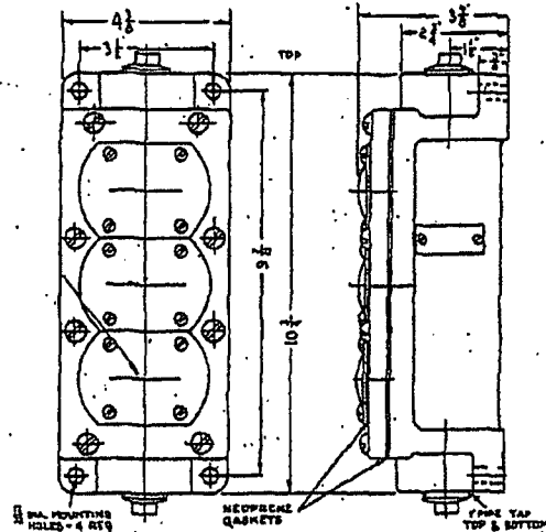
Three Unit Pushbutton Station using heavy duty momentary contact elements, rocker arm snap switches, standard duty momentary contact elements and indicating light elements.
