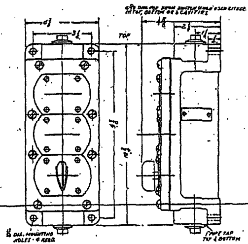
Three unit heavy duty master station with rotary drum switch element used in at least one unit. (Rotary drum switch element determines the maximum depth).
