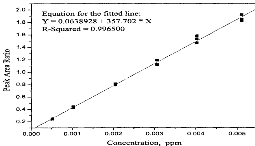
Figure 1a: Calibration curve showing linear fit (line) to replicate peak area ratio (squares) for calibration solutions of PFOA diluted with NANOpure deionized water and matrix matched over a concentration range of 0.00051 to 0.00511 ppm.
