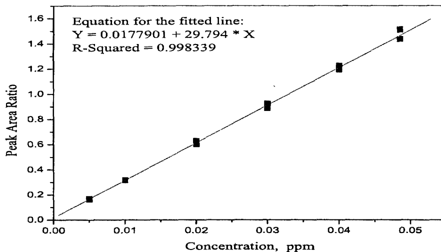
Figure 1b: Calibration curve showing linear fit (line) to replicate peak area ratio (squares) for calibration solutions of PFOA diluted with NANOpure deionized water and matrix matched over a concentration range of 0.0050 to 0.0485 ppm.
