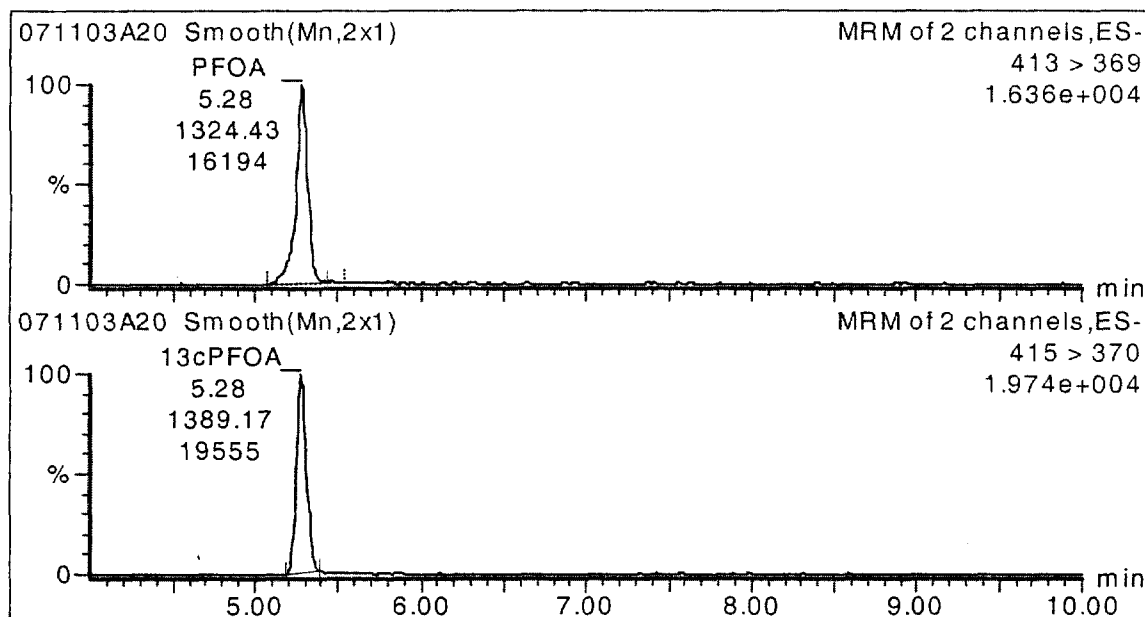
Figure 2d: Representative LC/MS chromatogram of PFOA analytical reference standard (0.00306 ppm) with the internal standard (0.0032 ppm). Negative ion/PFOA retention time is approximately 4.9 to 5.2 minutes.
