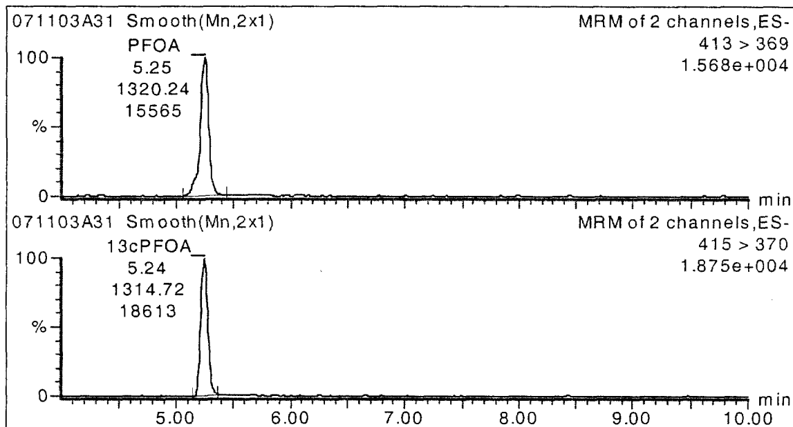
Figure 2e: Representative LC/MS chromatogram of 0.6 mg/mL dosing solution diluted to nominal concentration of 0.003 ppm of PFOA for negative ion /PFOA with retention time 5.2 minutes. The measured concentration of the representative solution is 0.613 mg/mL.
