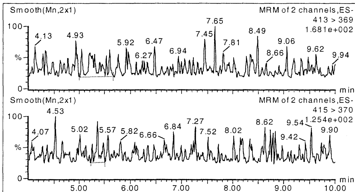
Figure 2a: Representative LC/MS chromatogram of NANOpure deionized water (sample diluent) used in the study. Negative ion/ perfluorooctanoic acid (PFOA) retention time is approximately 4.9 to 5.2 minutes.
