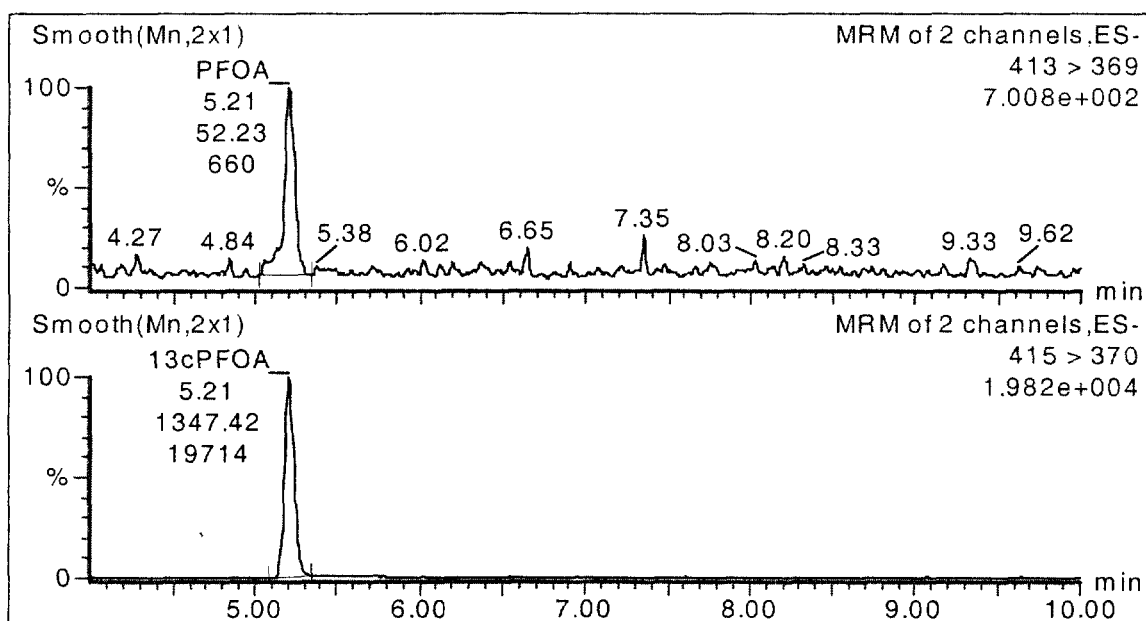
Figure 2b: Representative LC/MS chromatogram of NANOpure deionized water (sample diluent) used in the study with the internal standard. Negative ion/PFOA retention time is approximately 4.9 to 5.2 minutes.
