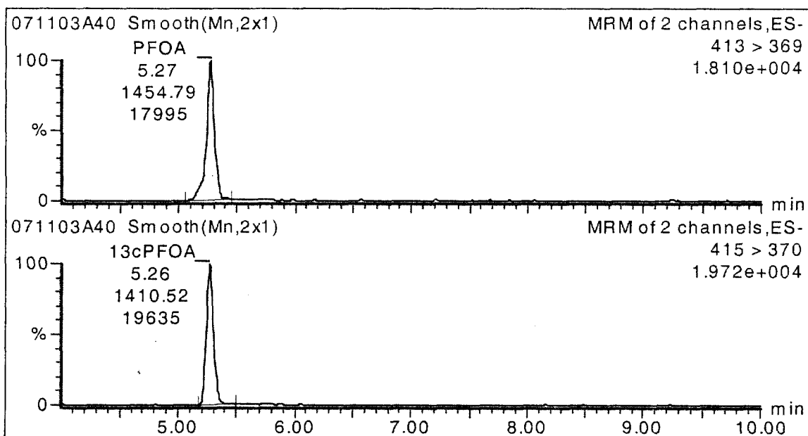
Figure 2f: Representative LC/MS chromatogram of low recovery dosing solution (0.584 mg/mL) diluted to nominal concentration of 0.003 ppm of PFOA for negative ion /PFOA with retention time approximately 5.2 minutes. The measured concentration of the representative recovery solution is 0.620 mg/mL.
